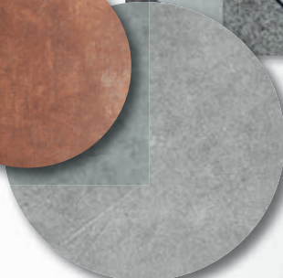
Oxide Texture
